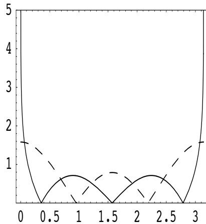
Figure 4: |\xi_{2,0}(\theta)| and |\Theta_{2,0}(\theta)| (dashed) as function of \theta .
