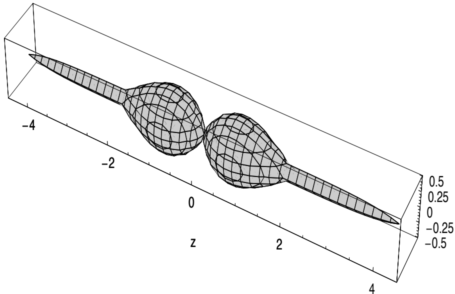
Figure 3: A boundary surface of |\Xi_{n=1,\ell=0,0}(r, \theta, \phi)|^2 .
