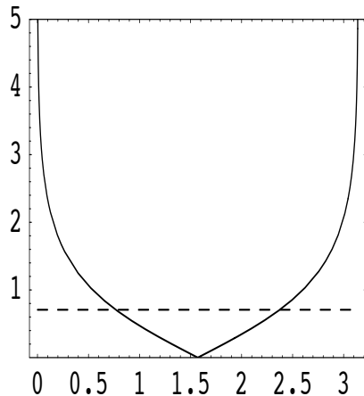
Figure 2: |\xi_{0,0}(\theta)| and |\Theta_{0,0}(\theta)| (dashed) as function of \theta .
