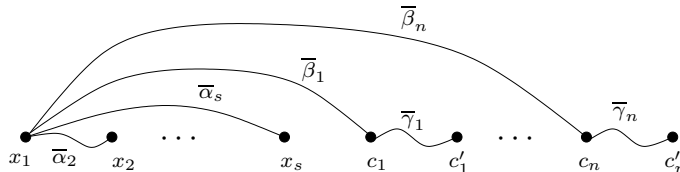
FIGURE 1. The class C and the chosen paths.
